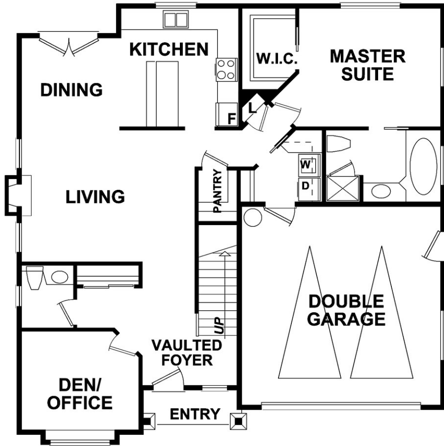
MAIN FLOOR AND GARAGE 1163 SQ FT
